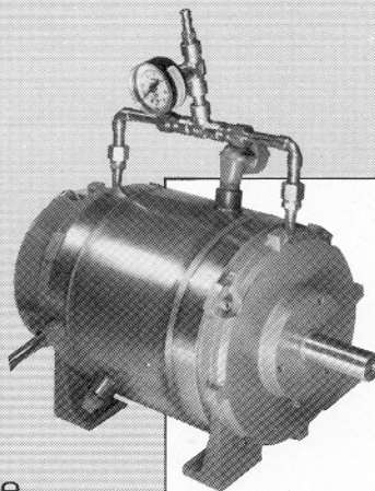
50 hp, 25,000 rpm 184T, liquid cooled, oil mist lubrication, 4 pole, 208V/ 833HZ test stand drive
