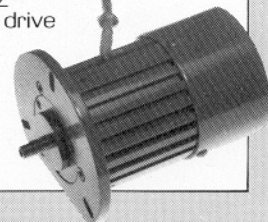
.3 hp, 24,000 rpm, 200V/400HZ power train drive
